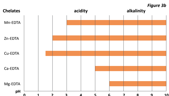
Figure 3. pH stability of several nutrient-chelate combinations under practical agricultural conditions where calcium is present. Figure 3a refers to iron chelates and Figure 3b to other chelates.
